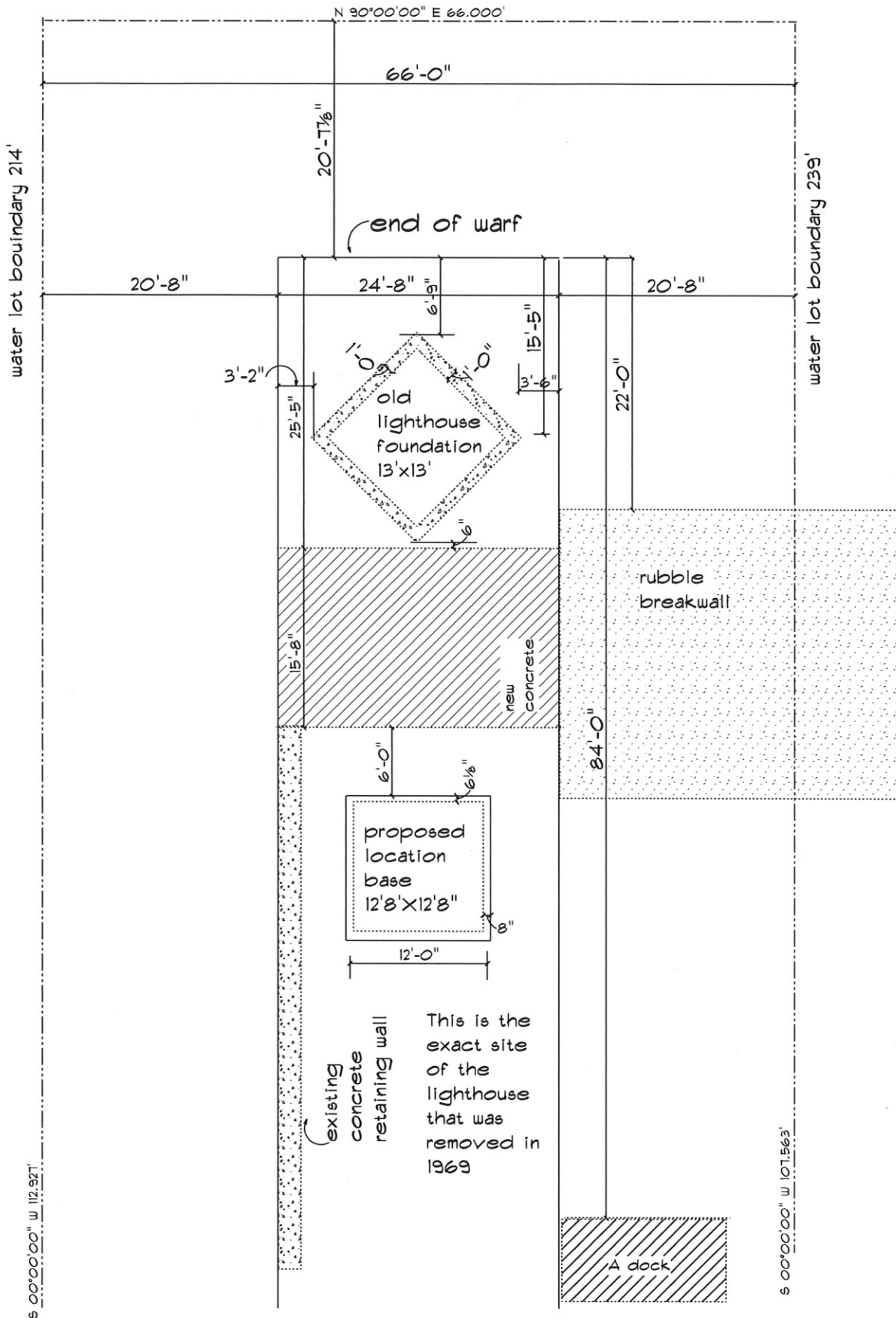
Concept Dwg. L. H. Lighthouse 2020 Site Plan Scale 1"=10' Drawn by: D. Hill
